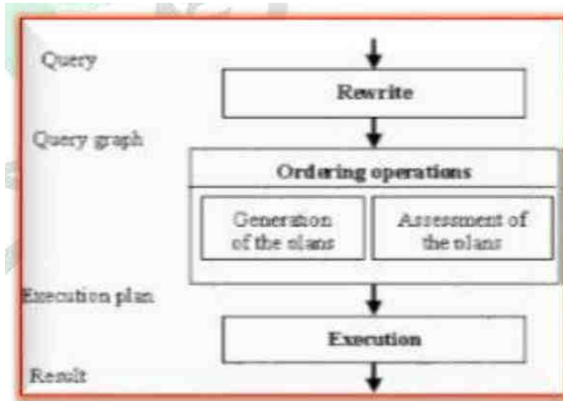
Fig.1- Optimisation process
