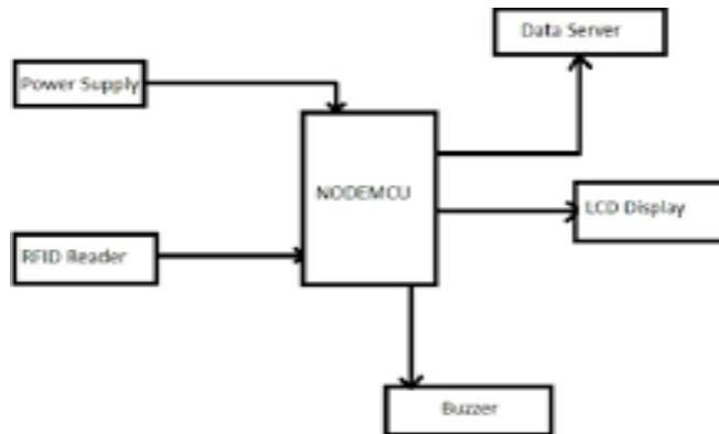
Fig.3-Block diagram for RFID based Intelligent Shopping Cart System
